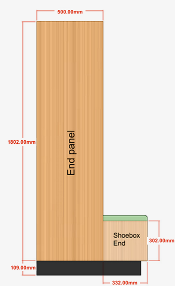
G Style seat with 40mm padded upholstery Open shoe storage shown
